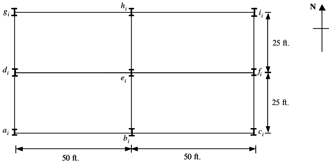
Figure 8. Structural floor plan
